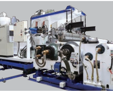
Extruder with Automatic T-Die & Casting Unit
